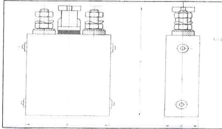
Fig. 1: Prismatic cell with two terminals and four lug (IEC 60623)
